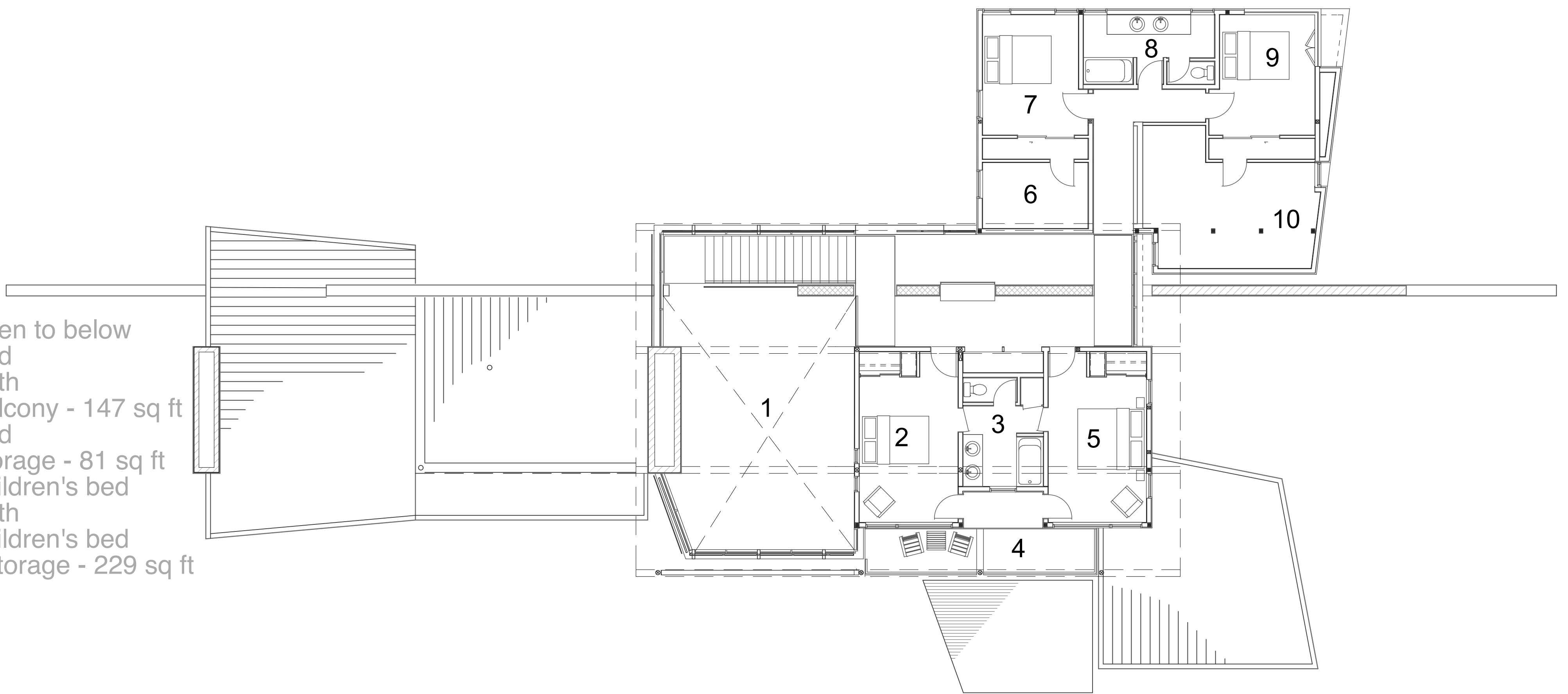
UPPER FLOOR PLAN
